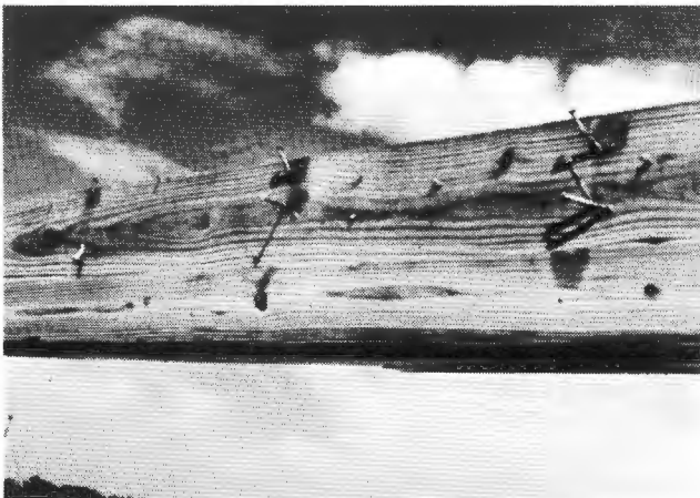
Figure 4.26. Toe Nailing Provides Limited Pull-Out Resistance
