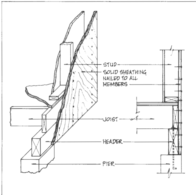
Figure 4.45. Plywood Anchorage
