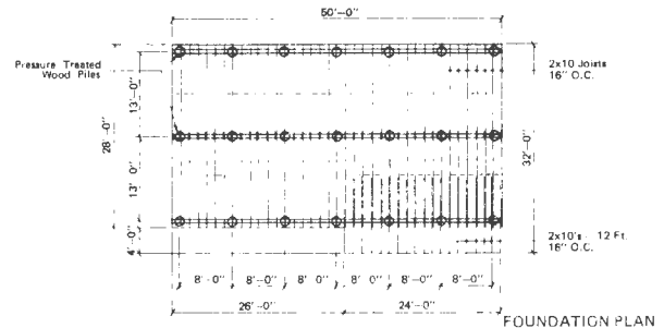
FOUNDATION PLAN
