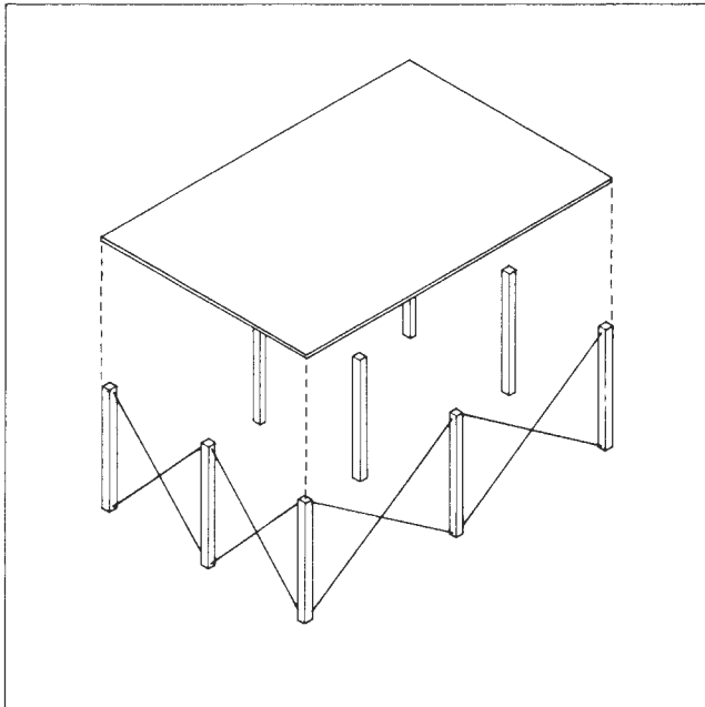
Figure 4.22. Diagonal Bracing
