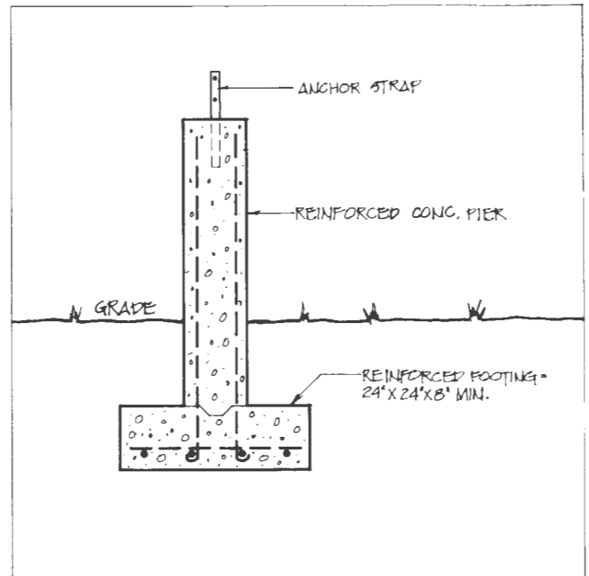
Figure 4.19. Reinforced Concrete Pier
